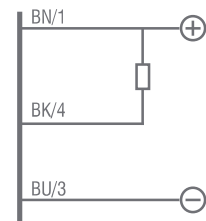
NPN Cable & M8 Plug Exit
