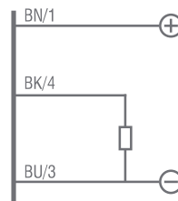
PNP Cable & M8 Plug Exit
