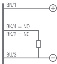
PNP Cable & M12 Plug Exit
