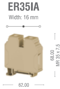
35 mm 2 Feed Through Terminal Block Insulated, Allen Key For 35mm DIN Rail
