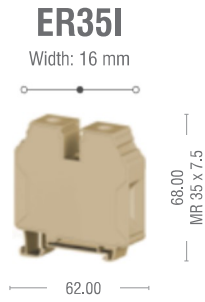
35 mm 2 Feed Through Terminal Block Insulated For 35mm DIN Rail
